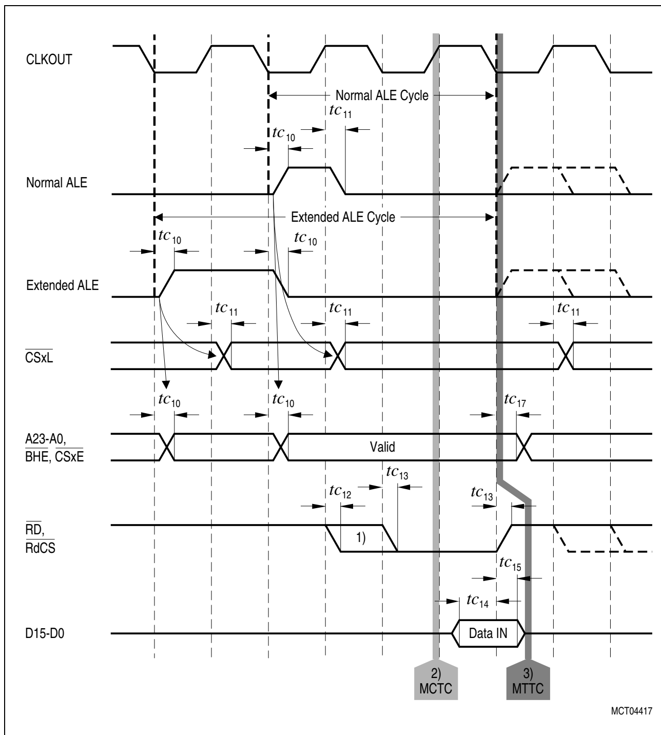
Figure 16 Demultiplexed Bus, Read Access
